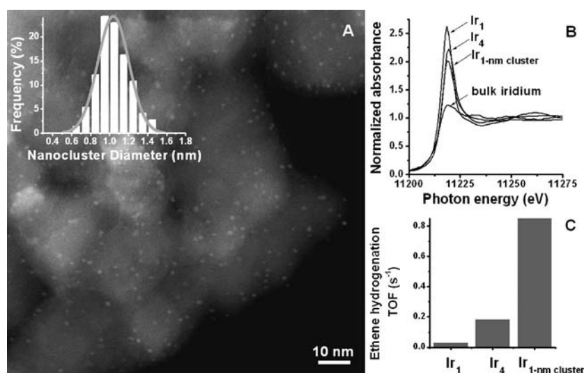
Figure 1. Characterization and catalytic activity of a sample containing supported iridium nanoclusters prepared by treating \text{Ir}(\text{C}_2\text{H}_4)_2 complexes on MgO in flowing \text{H}_2 at 673 K for 8 h. A) High-angle annular dark-field (HAADF) STEM image and histogram showing the distribution of nanocluster diameters (inset). B) Normalized XANES spectra at Ir L_{\text{III}} edge characterizing supported iridium complex, \text{Ir}_4 clusters, iridium clusters with an average diameter of approximately 1 nm, and iridium metal. C) Rate of ethene hydrogenation catalyzed by supported iridium complexes, \text{Ir}_4 clusters, and iridium nanoclusters with an average diameter of approximately 1 nm.
