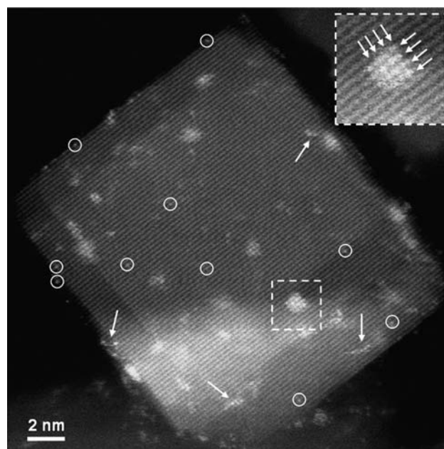
Figure 2. HAADF-STEM image of MgO-supported iridium species formed by the reaction of \text{Ir}(\text{C}_2\text{H}_4)_2(\text{acac}) with the MgO surface followed by exposure to the electron beam (the imaging dose was approximately 10^5 \text{ e}^- \text{ \AA}^{-2} ) for 30 s. Examples of isolated Ir atoms are encircled; the arrow indicates aligned Ir atoms en route to cluster formation. A magnified view of the cluster in the square frame is shown in the inset.
